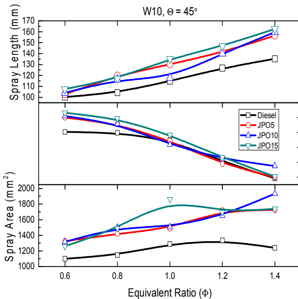
Figure 7: Comparison of spray characteristics of fuels at W10
