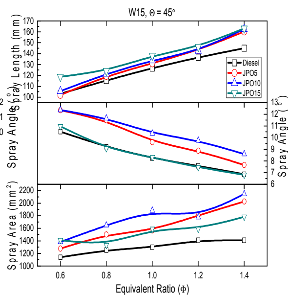
Figure 8: Comparison of spray characteristics of fuels at W15
