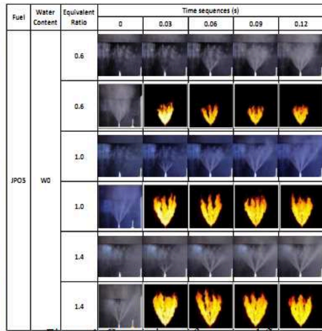
Figure 4: Comparison of spray and flame development for JPO5 at W0.
