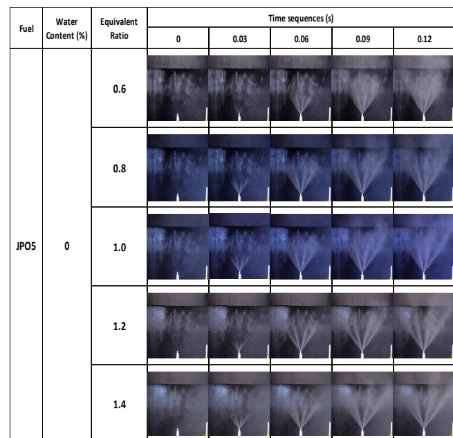
Figure 2: JPO5 biodiesel spray development (W0)
