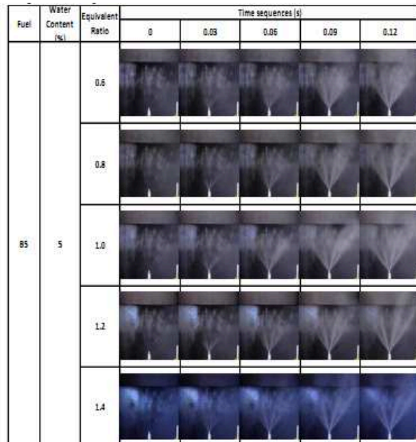
Figure 3: JPO5 biodiesel spray development (W5)
