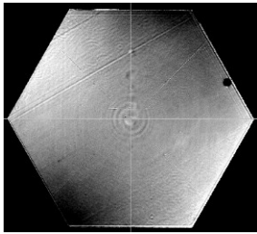
Fig. 9 SPN01 final phase-map, low order terms removed
