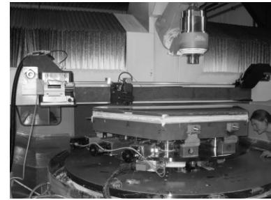
Fig. 3 NOM profilometer mounted on Zeeko machine
