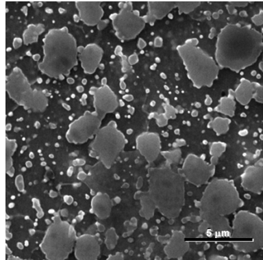
Fig. 1 Initial microstructure
