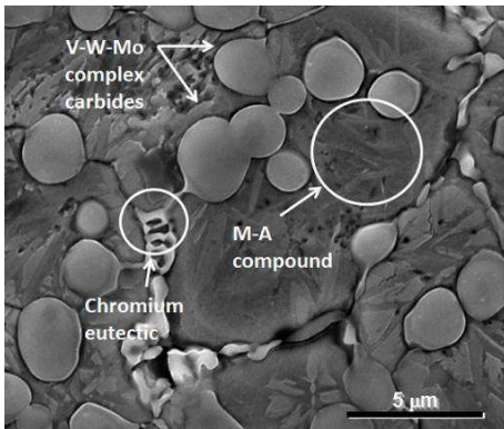
Fig. 4 Microstructure upon mini-thixoforming
