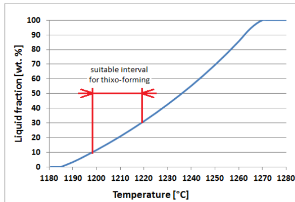
Fig. 2 Dependence of liquid fraction on temperature
