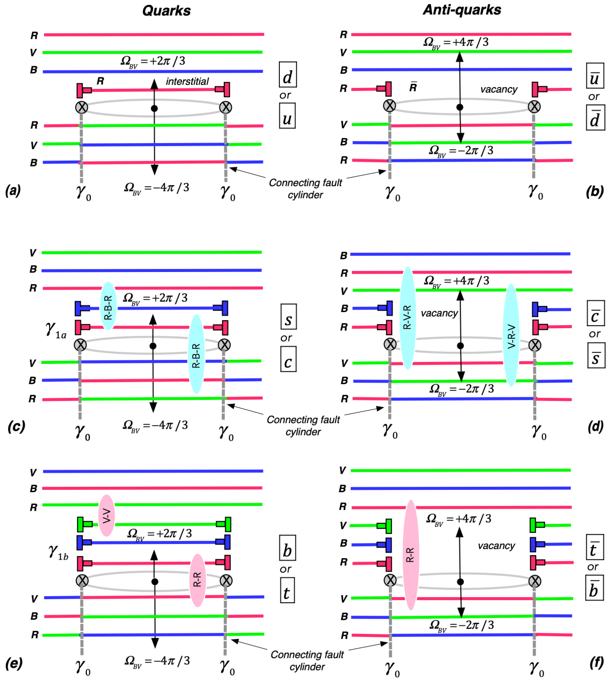
Fig. 39. The three families of quarks and anti-quarks obtained by adding or removing one or two dense planes, in combination with a screw disclination loop.
