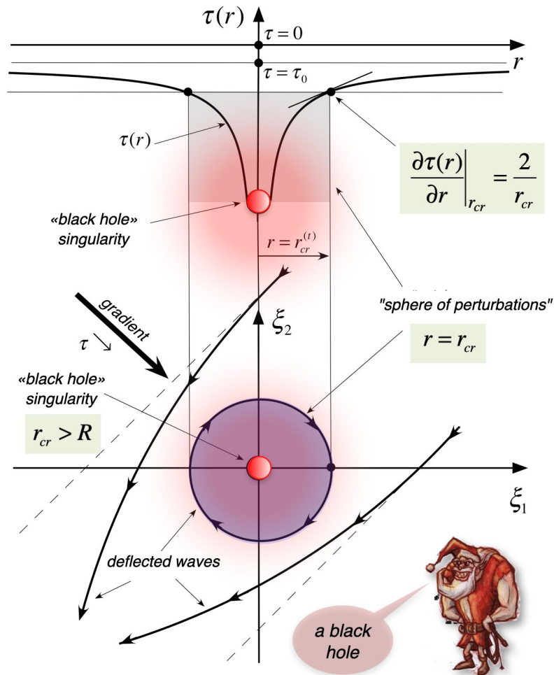
Fig. 9. The "sphere of perturbations", a real "black hole" in the vicinity of a negative singularity of expansion \tau
