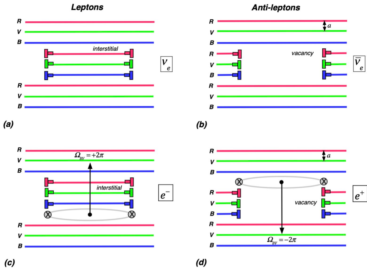
Fig. 35. Structure of the neutrino, the anti-neutrino, the electron and the positron, as assemblies of edge dislocation loops and screw disclination loops.
