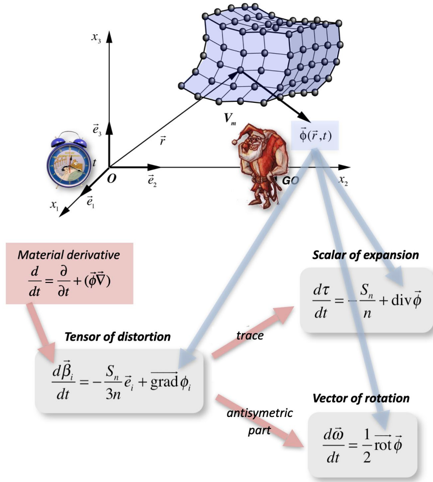
Fig. 1. Euler's coordinates and the geometro-kinetic equations
