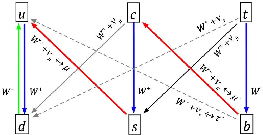
Fig. 40. Diagram of possible quark decays via weak interaction, with particles produced according to each decay pathway.
