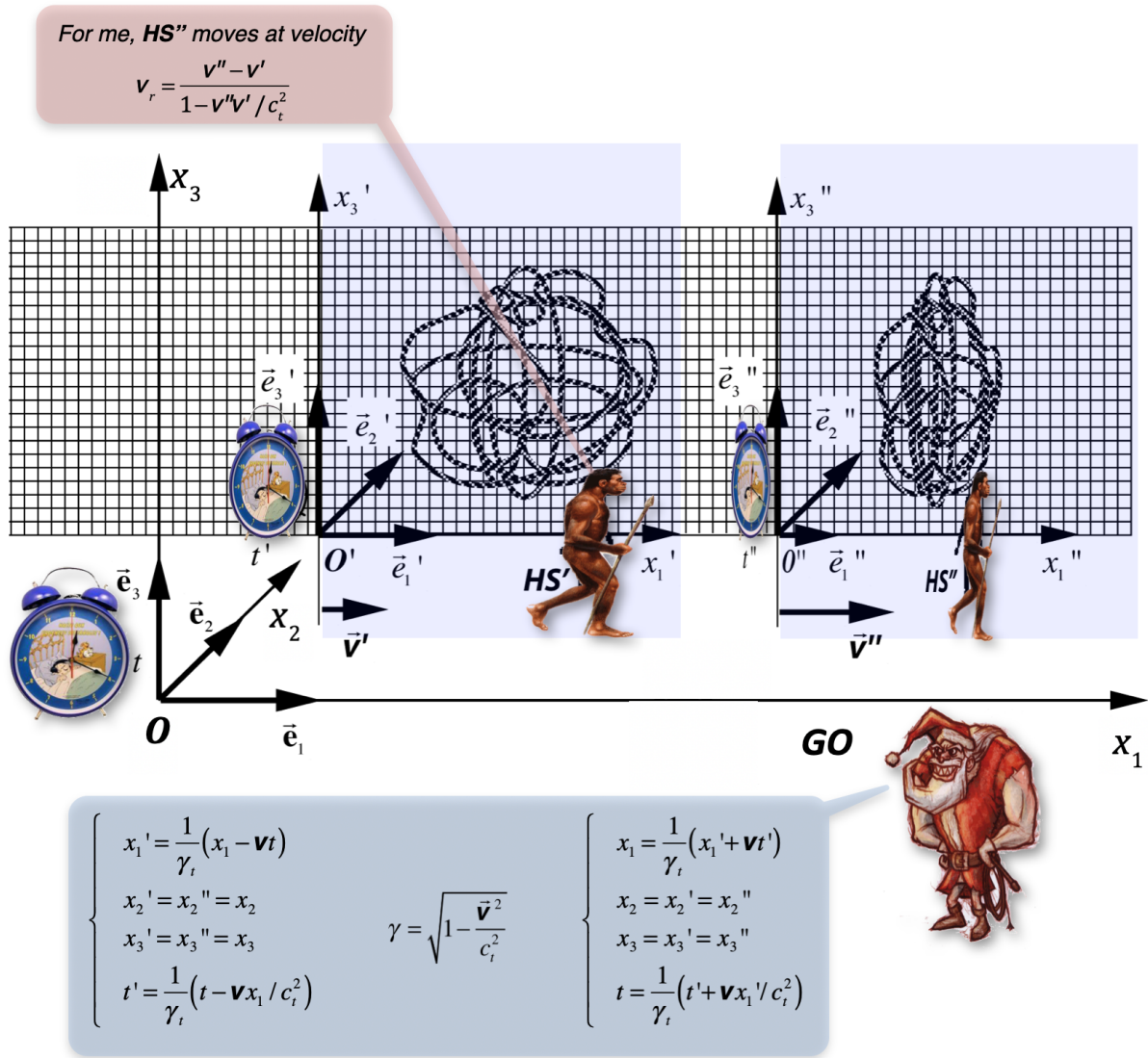
Fig. 12. The mobile Lorentz frames of the moving Homo Sapiens observers HS' and HS''
