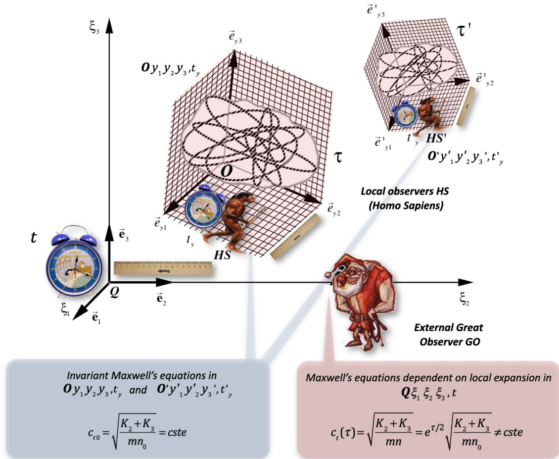
Fig. 15. Local rulers and clocks in the reference frames of the homo sapiens HS and HS' , and the local invariance of the Maxwell's equations in the HS frames.
