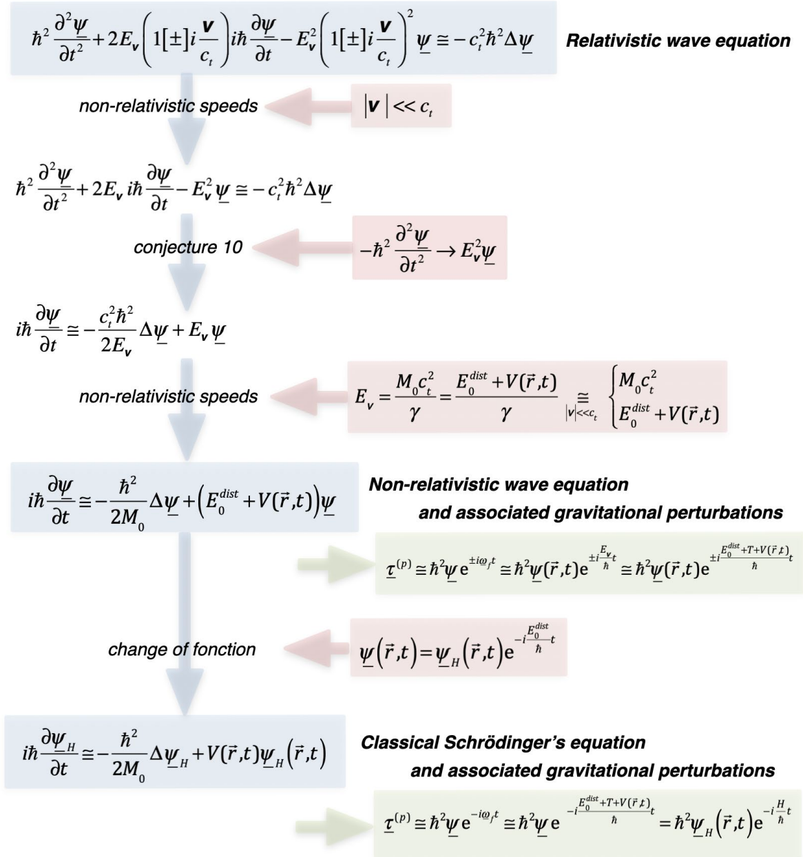
Fig. 24. Non-relativistic wave equation and Schrödinger's equation in the case of gravitational perturbations associated to a massive singularity moving at non-relativistic speed
