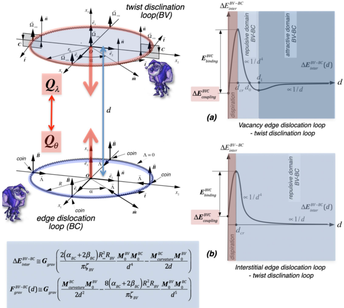
Fig. 17. Long and short range interactions potential between a twist disclination loop (BV) and an edge dislocation loop (BC), with different dislocation loops nature
