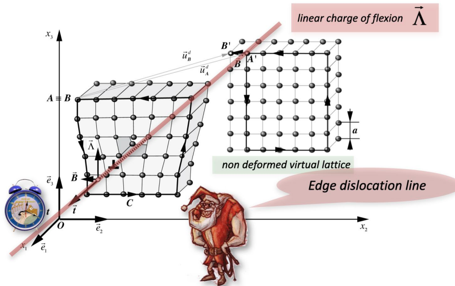
Fig. 4. Edge dislocation line quantified in a cubic lattice
