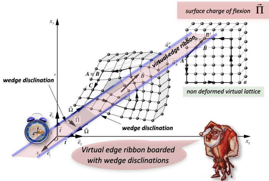
Fig. 6. Doublet of quantified wedge disclinations with the formation of a virtual edge dislocation ribbon
