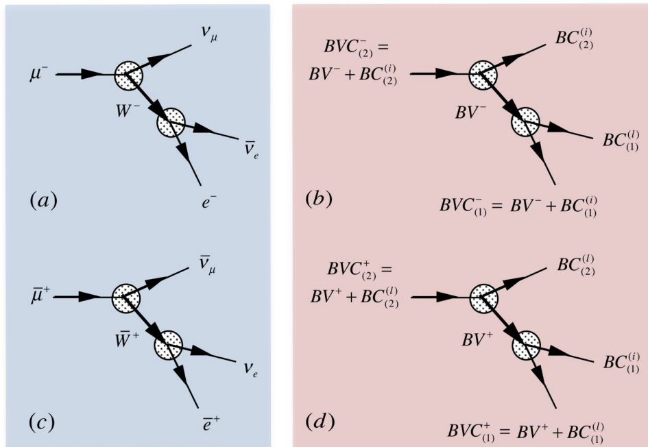
Fig. 18. Analogy between the weak leptonic interaction (a) and (c) and the decompositions and recompositions of dispiration loops (b) and (d)
