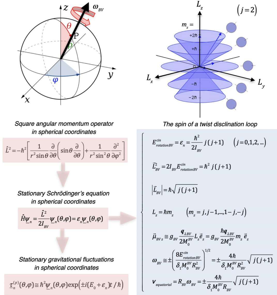
Fig. 28. Quantum solution of rotation of the twist disclination loop: quantified rotational energy levels and magnetic quantum number
