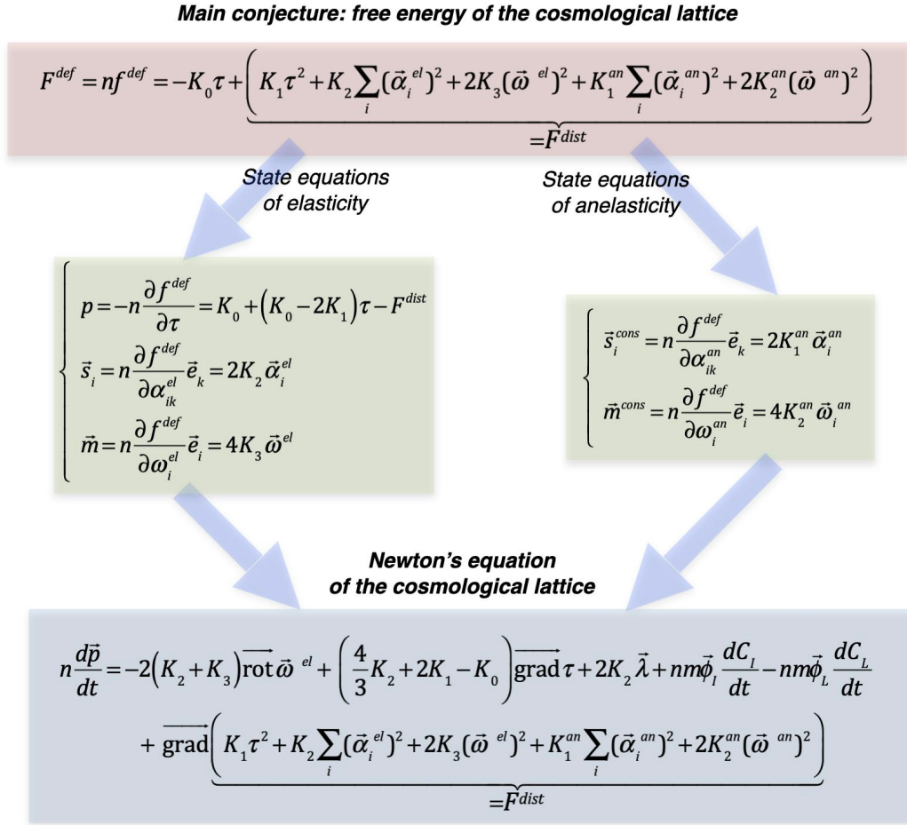
Fig. 7. The main conjecture which leads to the cosmological lattice and its Newton's equation
