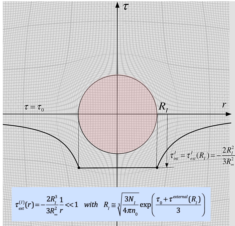
Fig. 20. The internal and external expansion fields of a macroscopic interstitial
