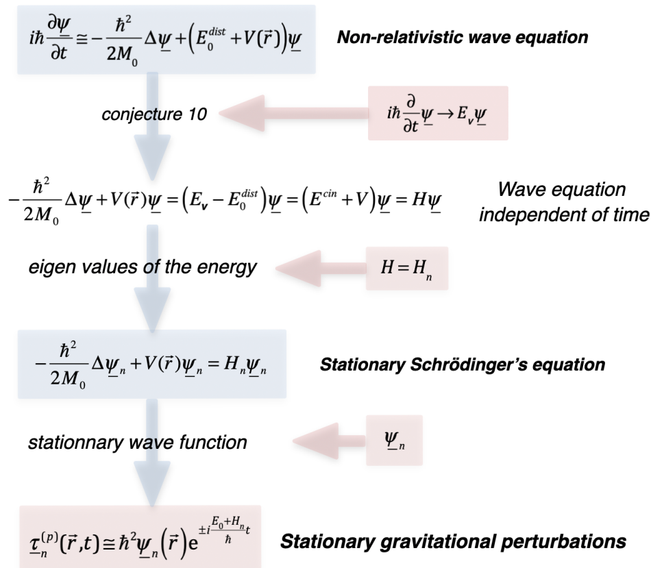
Fig. 25. Schrödinger's standing wave equation with eigenvalues for a massive singularity placed in a static potential
