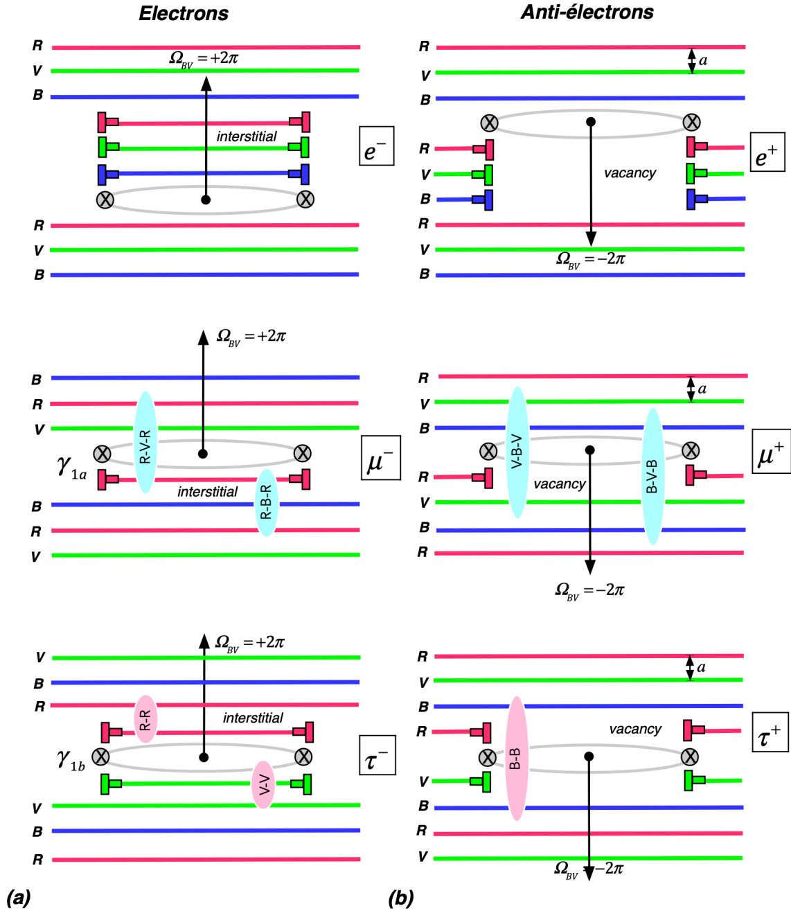
Fig. 38. The three families of electrons and anti-electrons obtained by removing or adding two or one dense plane, in combination with a screw disclination loop.
