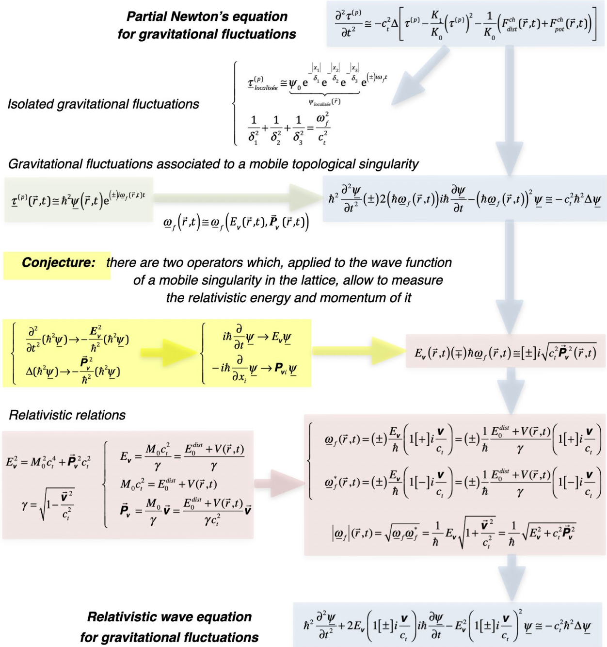
Fig. 22. From Newton's partial equation for gravitational fluctuations to the relativistic wave equation for the fluctuations associated with a moving singularity
