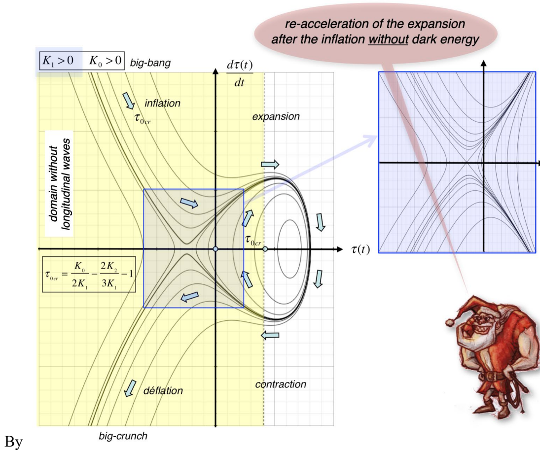
Fig. 10. «Cosmological behavior» of the speed of cosmological expansion d\tau/dt as a function of the expansion \tau of a cosmological lattice with K_1 > 0
