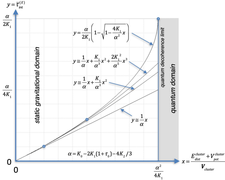
Fig. 13. The mean perturbation field in the static solution domain for energy density values of the singularity below the critical value, and domain of the quantum behaviour for values above the critical value.
