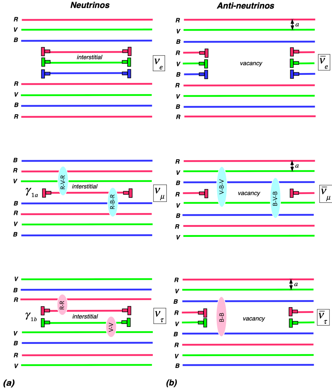
Fig. 37. The three families of neutrinos and anti-neutrinos obtained by removing or adding one or two dense planes, with the appearance of stacking faults of type X-Y-X and X-X .
