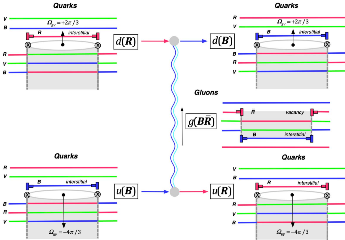
Fig. 31. Feynman diagram of the color exchange of two quarks by the exchange of a bicolour gluon
