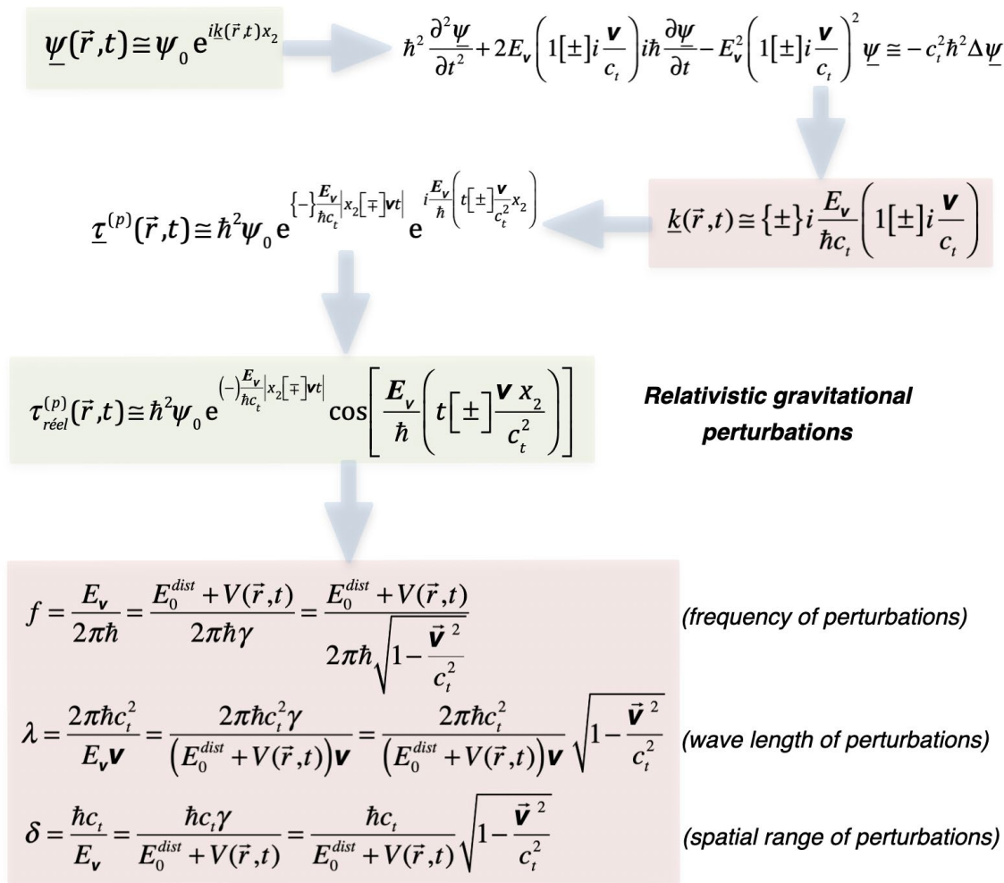
Fig. 23. Associated gravitational perturbations to a massive singularity moving at relativistic speed
