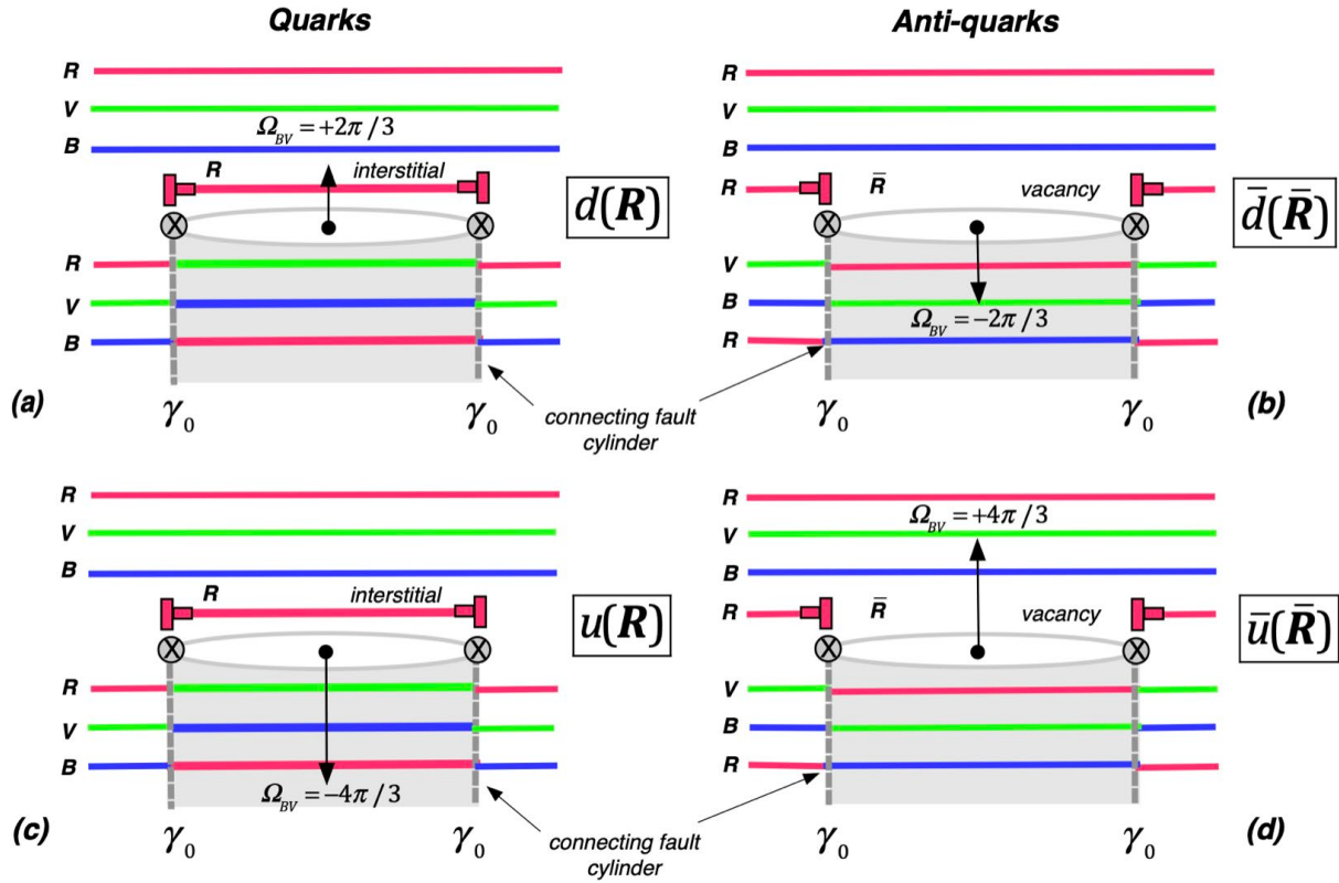
Fig. 29. Quarks and antiquarks formed by combinations of screw disclination loops of quantized angles with edge dislocation loops which ensure the continuity of succession of planes R,B,V .
