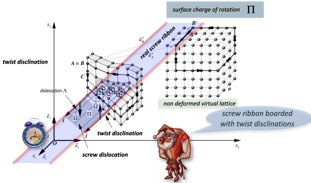
Fig. 5. Quantized two-dimensional dislocation ribbon composed of three screw lattice dislocations, with the formation of two virtual twist disclination lines
