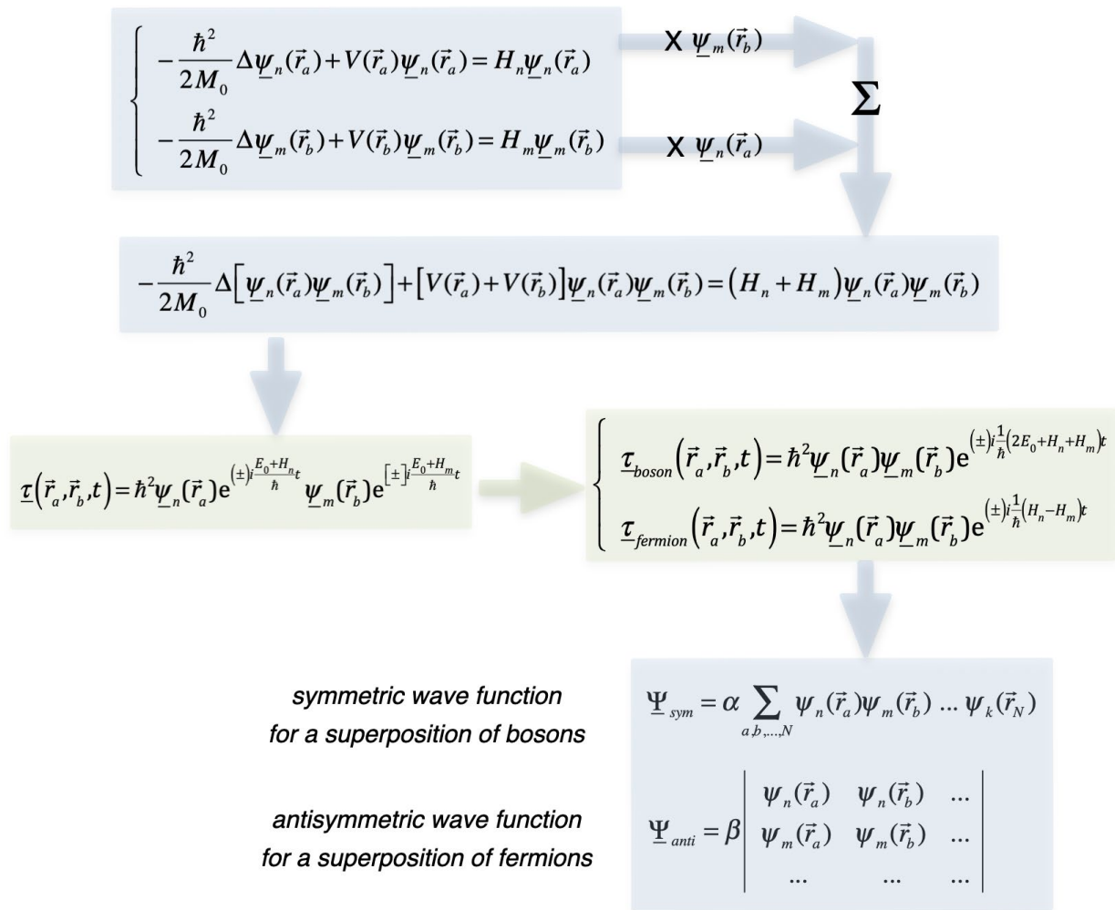
Fig. 26. Stationary equation for the superposition of topological singularities, gravitational fluctuations of bosons and fermions and symmetrical and anti-symmetrical wave functions
