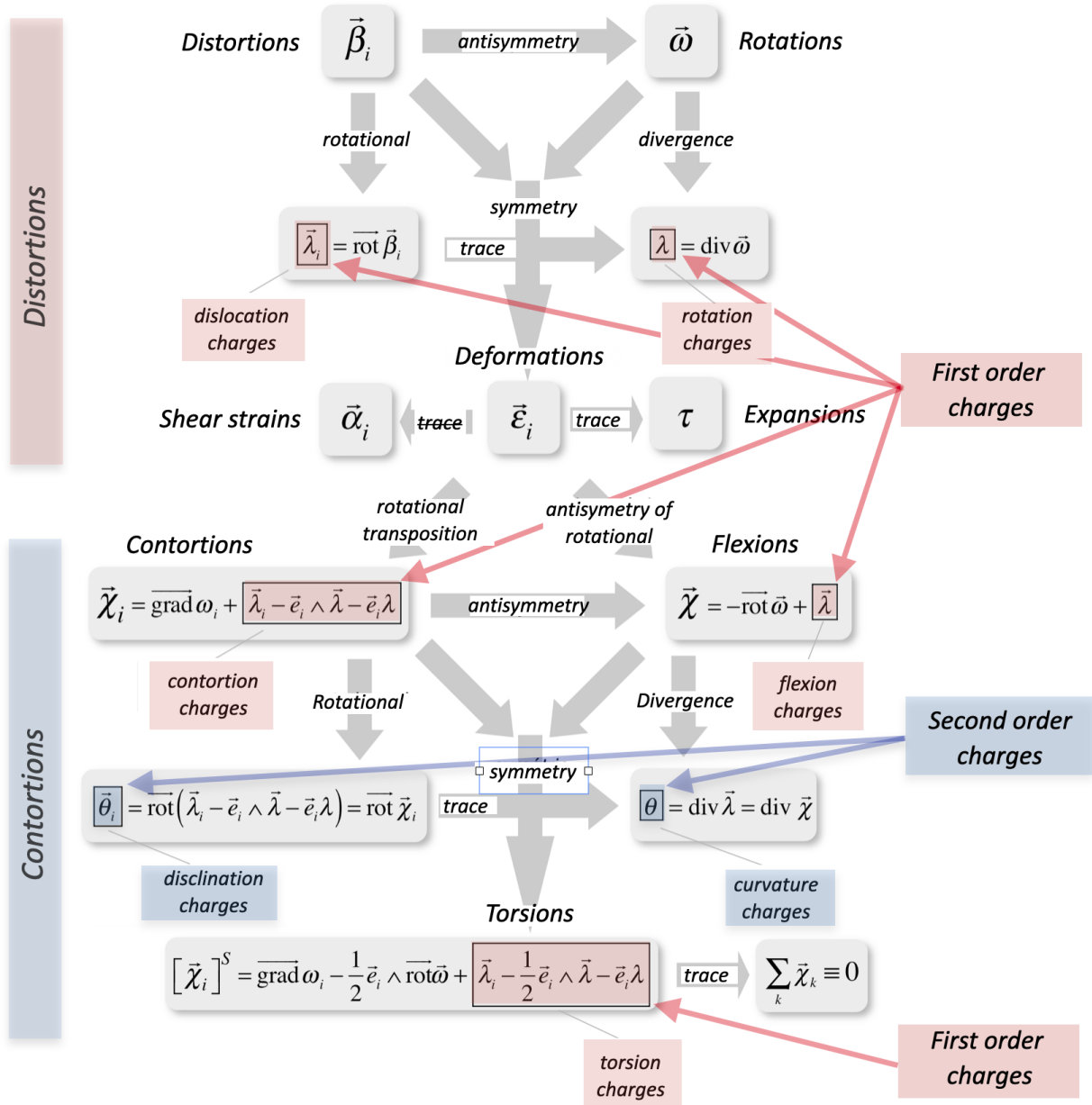
Fig. 2. The system of distortions and contortions in the presence of plastic charges and the geometro-compatibility equations
