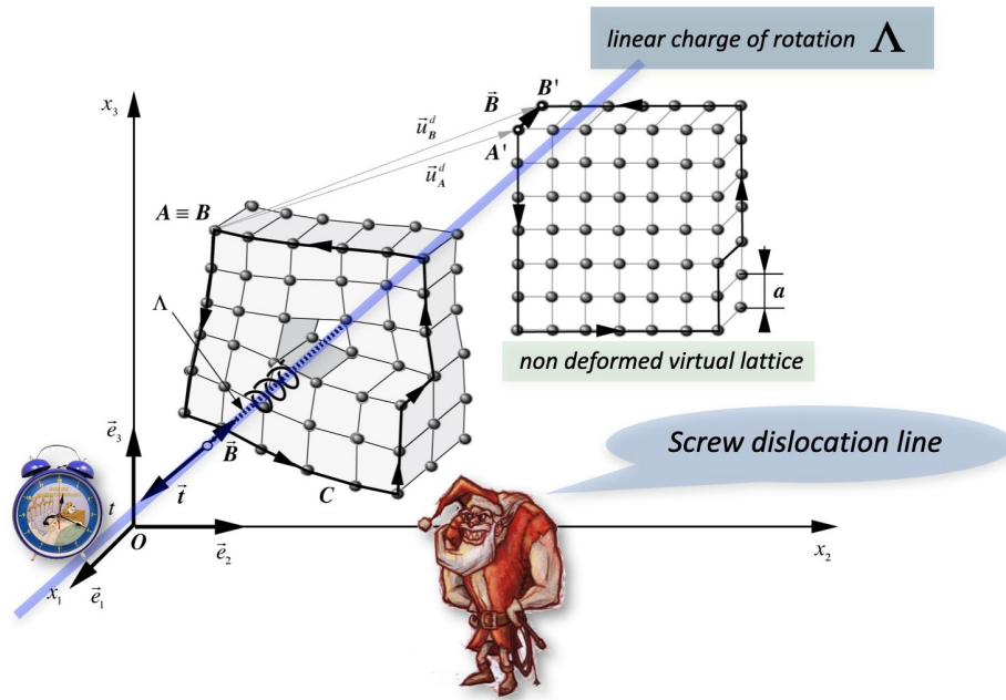
Fig. 3. Screw dislocation line quantified in a cubic lattice
