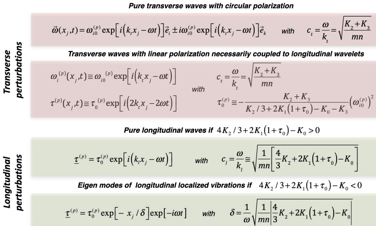
Fig. 8. Transverse and longitudinal perturbations in the cosmological lattice
