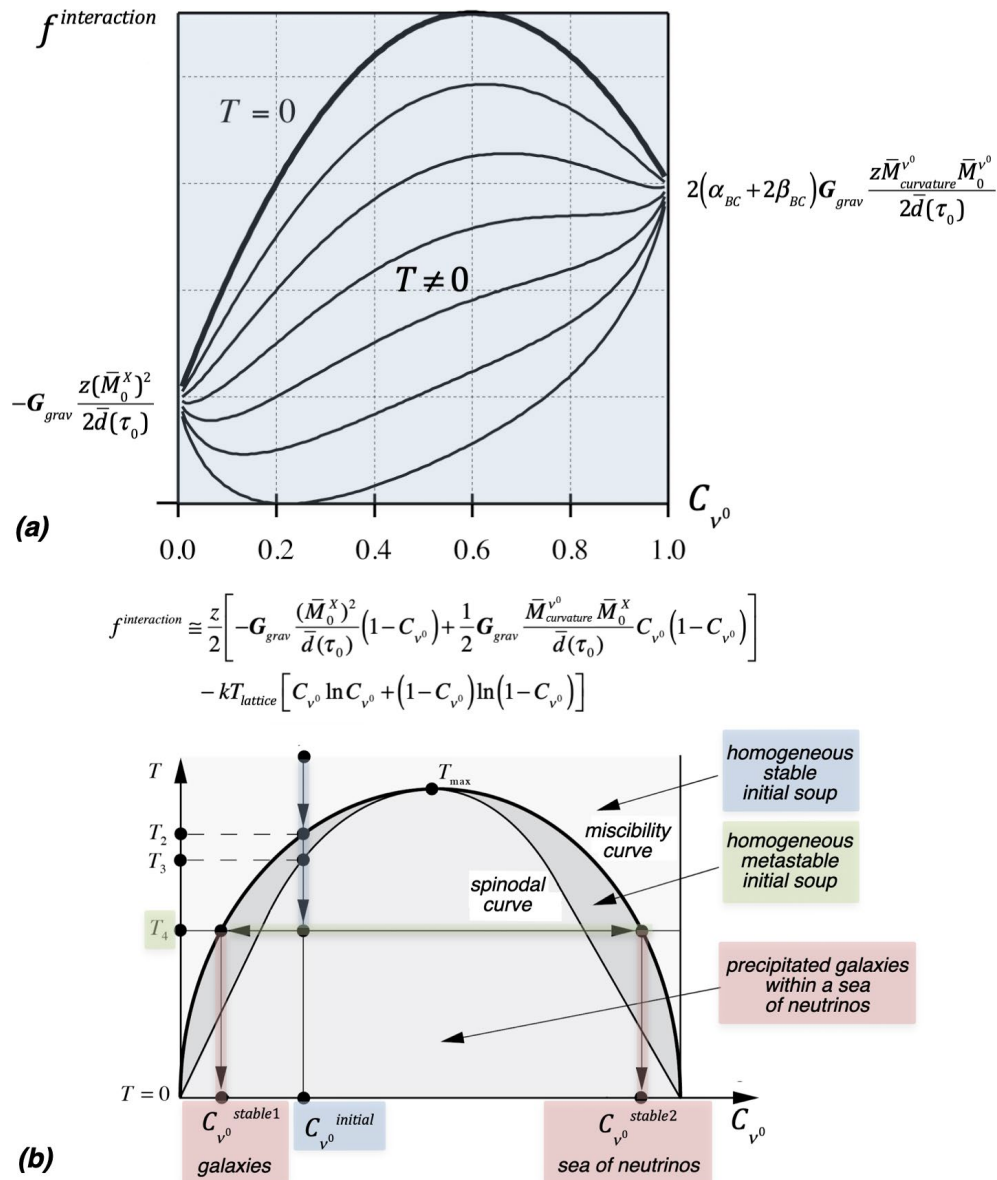
Fig. 21. (a) The particle free interaction energy within the initial hot soup of particles as a function of the concentration of repulsive neutrinos for different lattice temperatures (b) Phase diagram of matter in the Universe as a function of lattice temperature
