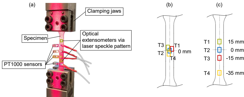
Figure 1. (a) Experimental setup for cyclic tensile tests; (b) PT1000 setup for measurement validation test; (c) general test setup;
