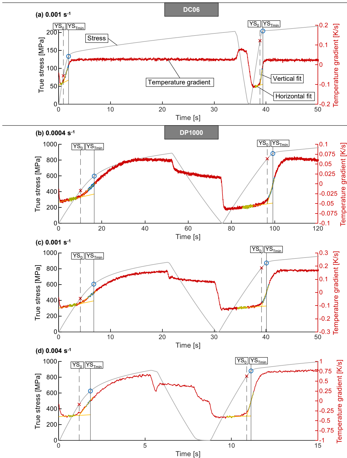
Figure 4. True stress versus time curve in comparison with the corresponding temperature gradient versus time curve for the materials (a) DC06 and (b-d) DP1000. Shown is the initial loading and the first unloading loading cycle. For DP1000 three different strain rates are shown (b-d).
