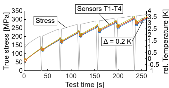
Figure 2. True stress versus time curve (strain rate 0.001 \text{ s}^{-1} ) and corresponding temperature signals (T1 – T4) for validation test setting (see Figure 3) for DC06.
