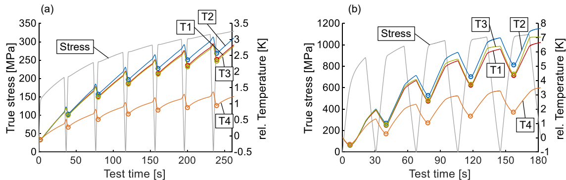
Figure 3. True stress versus time and temperature versus time curve for a cyclic tensile test (strain rate 0.001 \text{ s}^{-1} ) for (a) DC06 and (b) DP1000.
