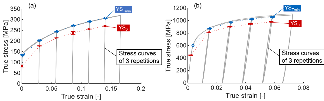
Figure 5. True stress vs. true strain curves (strain rate 0.001 \text{ s}^{-1} ) of three repetitions and the parameters YS_{Tmin} and YS_0 with standard deviation from temperature T_2 for (a) DC06 and (b) DP1000.
