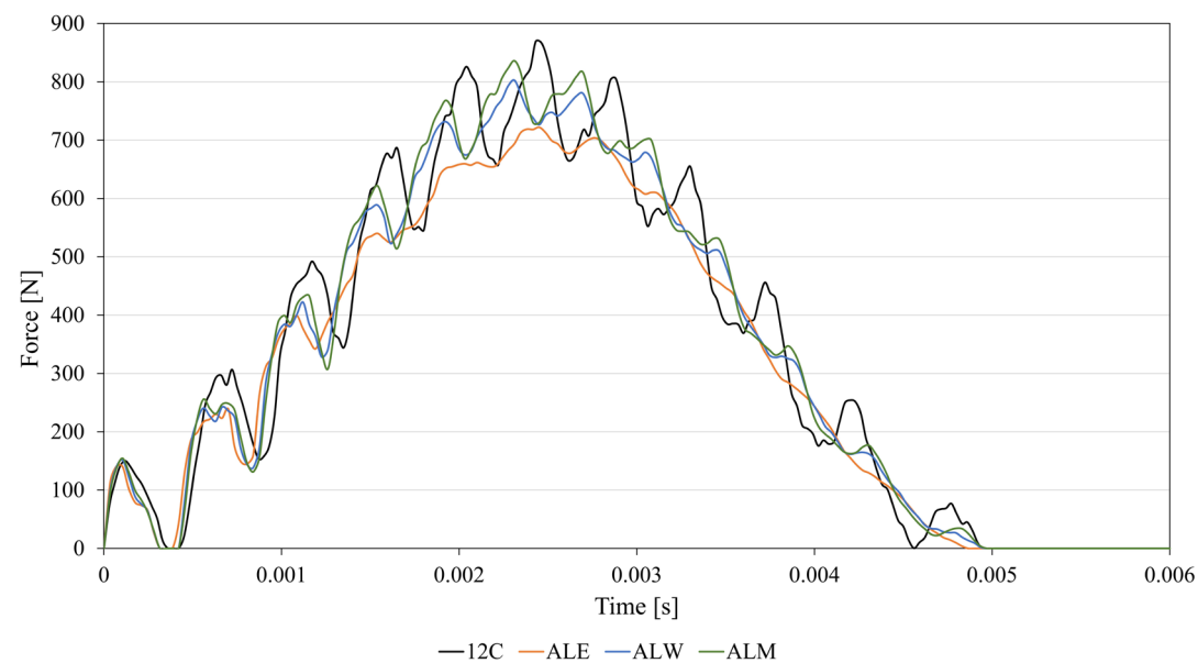
Figure 8: Contact force.
