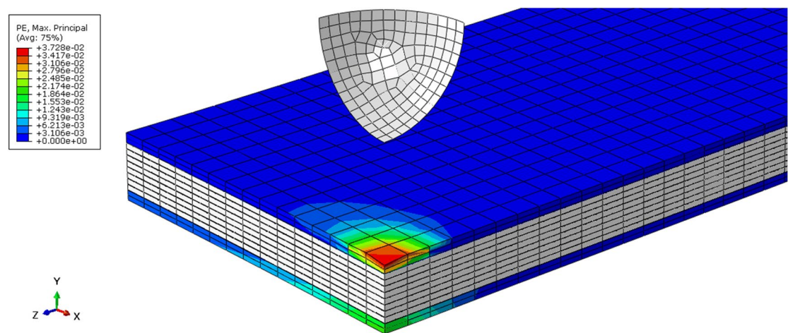
Figure 7: Residual strain in the Al layers in ALE model (composite layers and impactor are in white).
