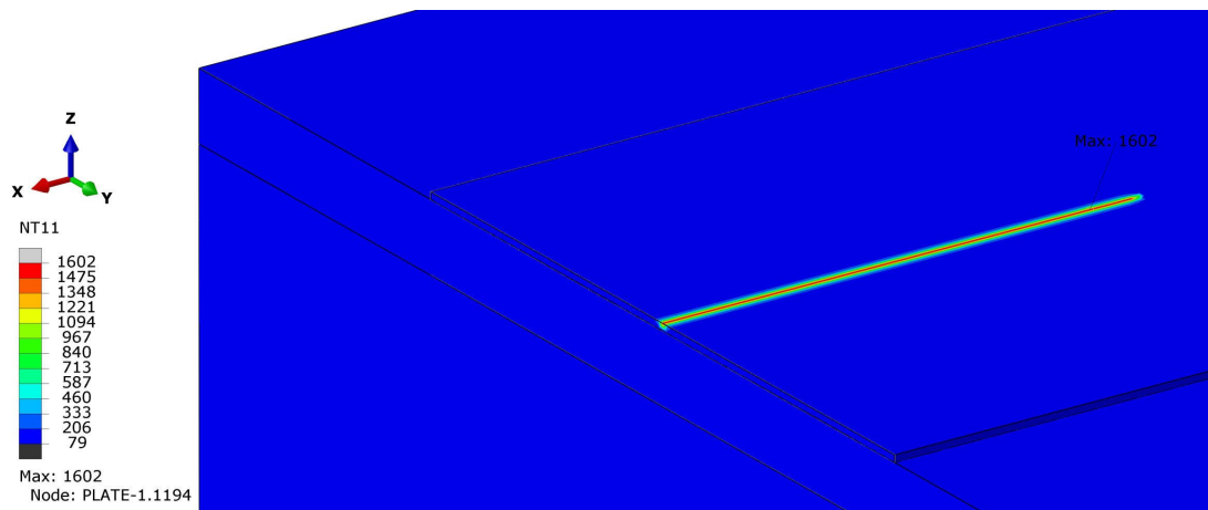
Figure 3: Nodal temperature predicted using time-increment=0.0028 s. Section cut at X=7 mm.
