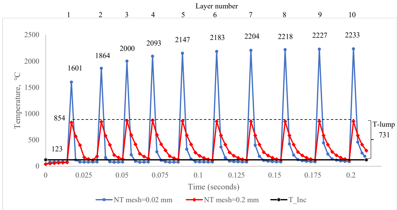
Figure 6: Summary of temperature prediction using one layer per element with 0.02 mm mesh and 10-layers lumped per element with 0.2 mm mesh.
