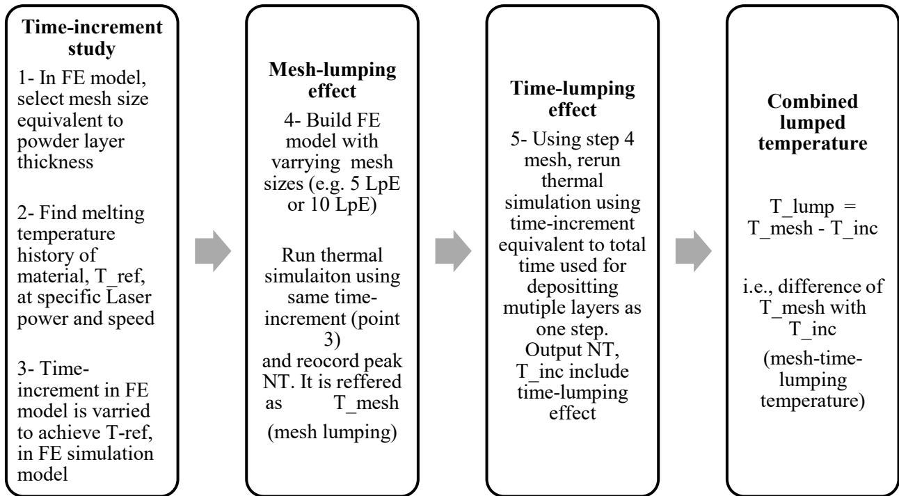
Figure 2: Methodology for predicting lumping temperature due to mesh size and time-increment effect.
