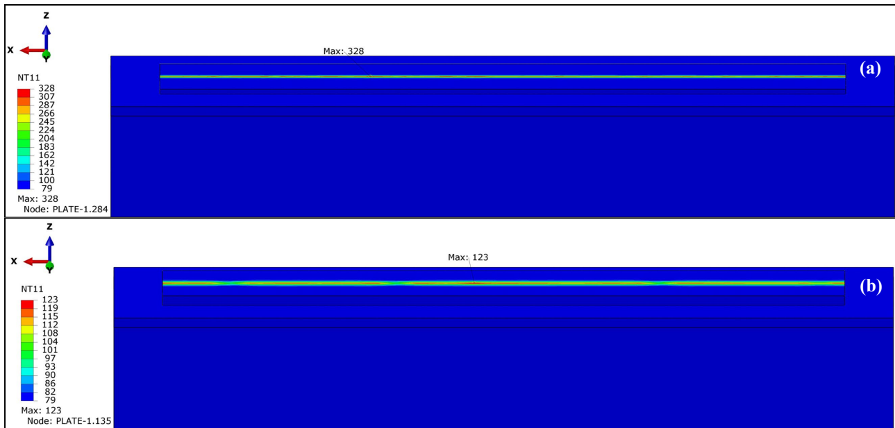
Figure 5: Temperature predicted using (a) lumped time for 5 layers=0.096489 and (b) lumped time for 10 layers= 0.208989.
