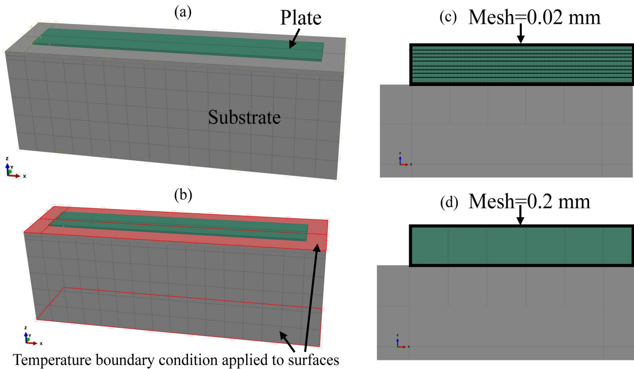
Figure 1: FE model (a) Plate (green) and substrate (grey) (b). Fixed temperature boundary condition applied in FE model (c). Ten separate powder layers with mesh size 0.02 mm per element (d). 10 combined layers lumped into one 0.2 mm element.
