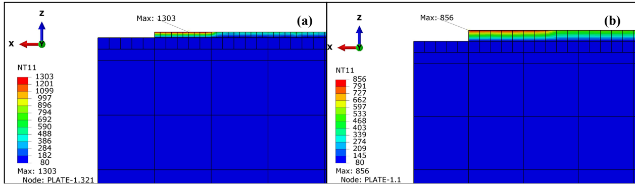
Figure 4: Temperature predicted using time-increment=0.0028 s for both cases: (a) 5LpE (b) 10LpE. Section cut at Y=1 mm.
