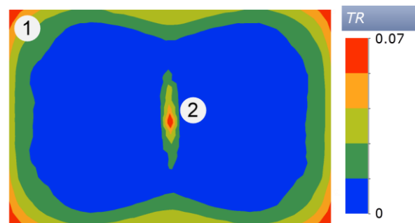
Fig. 4. Profile section with TR value (1) calculated for the design with evident underfilling defect
