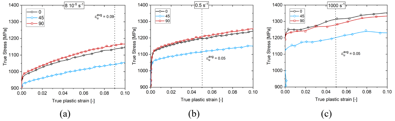
Fig. 4: True stress strain curves tensile experiments at 0°, 45° and 90° with respect to RD at low (a), intermediate (b) and high (c) strain rates ( 8 \cdot 10^{-5} , 0.5 and 1000 \text{ s}^{-1} ).
