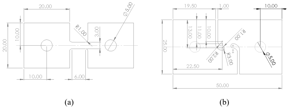
Fig. 1: Geometry tensile (a) and in-plane shear (b) samples used for quasi-static and intermediate velocity experiments. Dimensions are given in mm.
