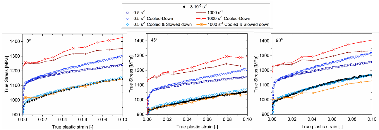
Fig. 6: Experimental hardening curves, and cooled-down and slowed-down curves obtained for intermediate and high strain rates experiments, for three different orientations (0°, 45° and 90° with respect to RD).
