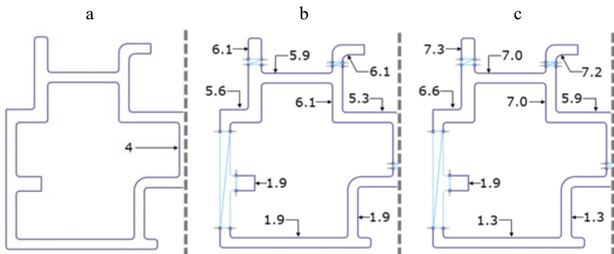
Fig. 5. Bearing maps for different designs: a – initial, b – intermediate, c – optimised
