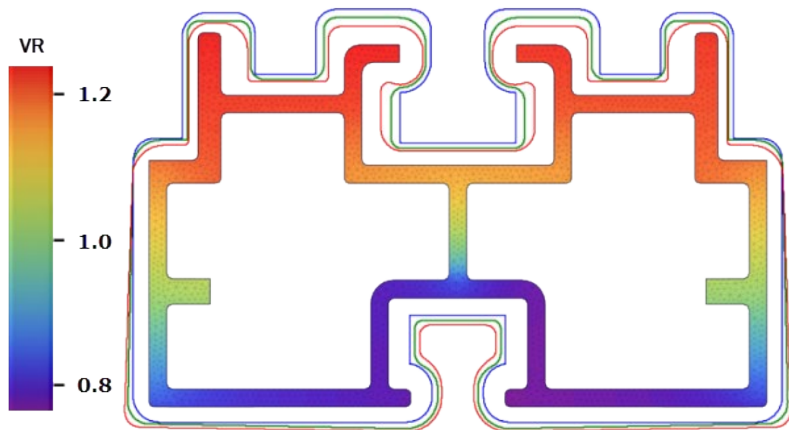
Fig. 7. Distribution of initial relative velocity (4) with prechamber contours: blue – initial, green – intermediate, red – optimised
