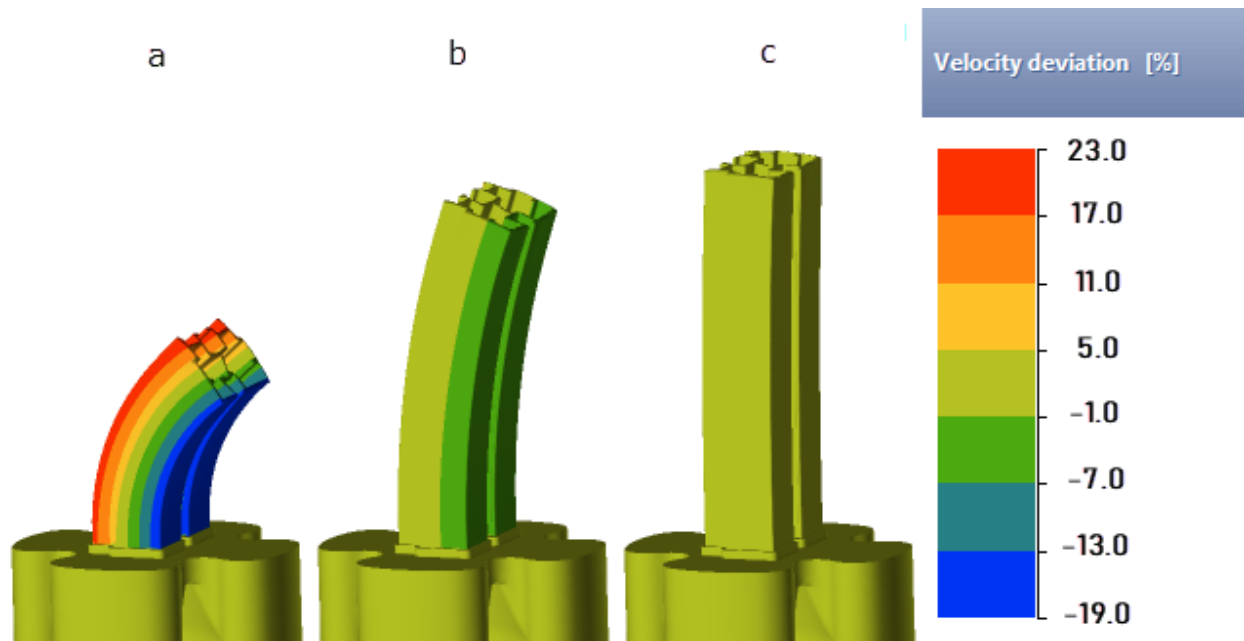
Fig. 4. Velocity deviation (3) distribution for different bearing designs: a – initial, b – intermediate, c – optimised
