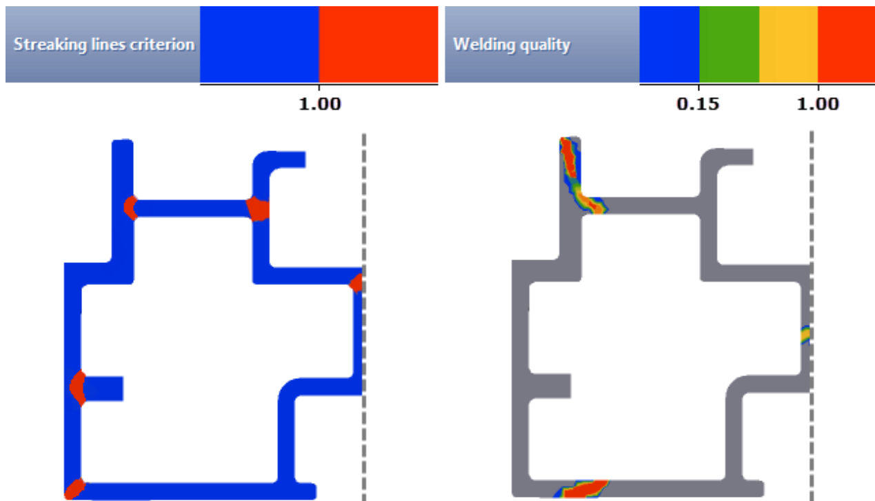
Fig. 8. Streaking lines (left) and welding quality (right) distributions calculated for the optimised design
