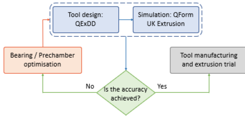
Fig. 2. Graphical representation of the optimisation integration of CAD and CAE
