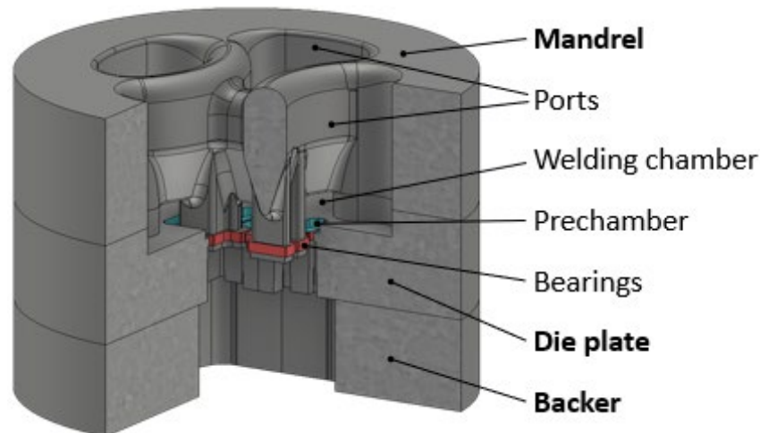
Fig. 1. Simplified representation of porthole die set for aluminium profile extrusion
