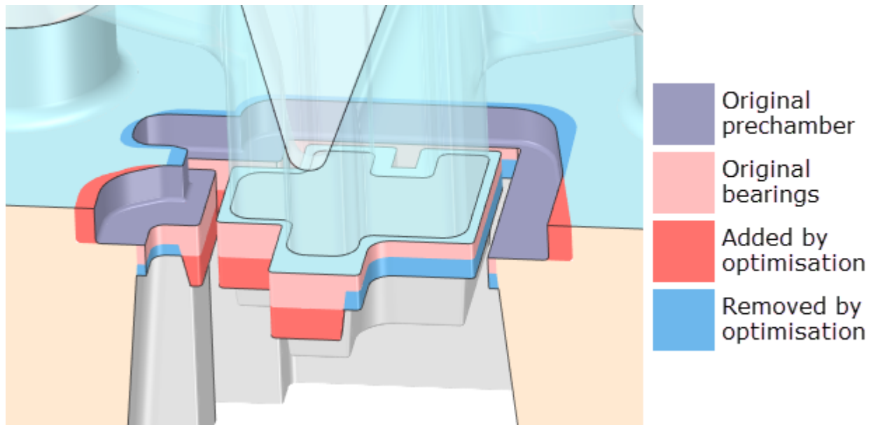
Fig. 3. On the explanation of optimisation procedure
