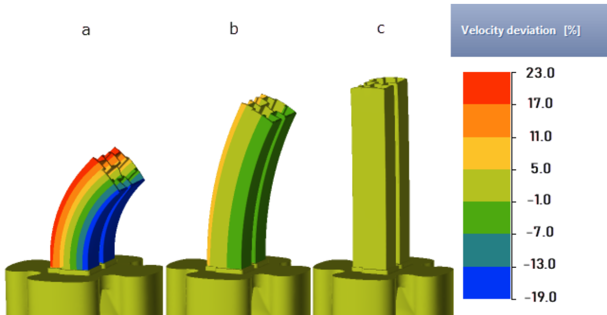
Fig. 6. Velocity deviation (3) distribution for different prechamber designs: a – initial, b – intermediate, c – optimised
