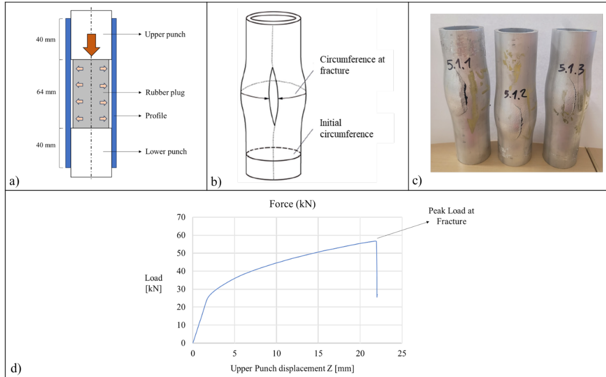
Fig. 15. a) Schematization of the bulge test, b) Initial circumference and circumference at fracture, c) Profiles after the bulge test, d) Force-Upper punch displacement graph.
