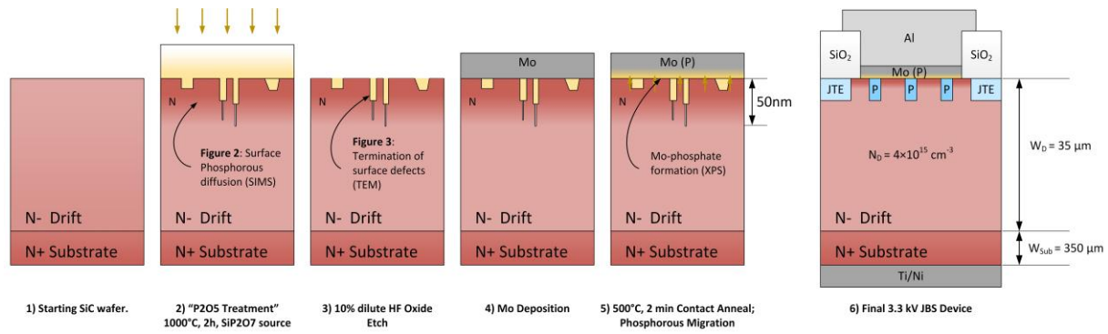
Figure 1: 1-5 show the processing steps carried out during the P_2O_5 treatment and Mo/SiC contact formation, and their effect on the Schottky interface. 6 shows the layout of the final 3.3 kV JBS diode.
