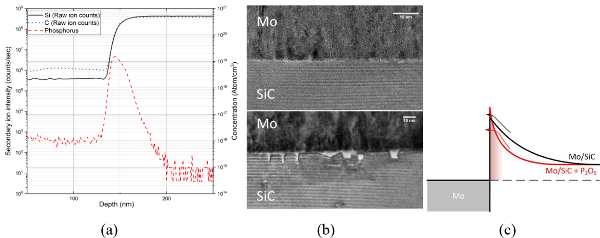
Figure 4: a) SIMS analysis showing the build-up of P at the P 2 O 5 treated Mo/SiC interface, b) HR-TEM images of the untreated (top) and P 2 O 5 treated (bottom) Mo/SiC interface [5], and c) Mo/SiC band diagrams, pre-and post-treatment, based on TCAD simulations.
