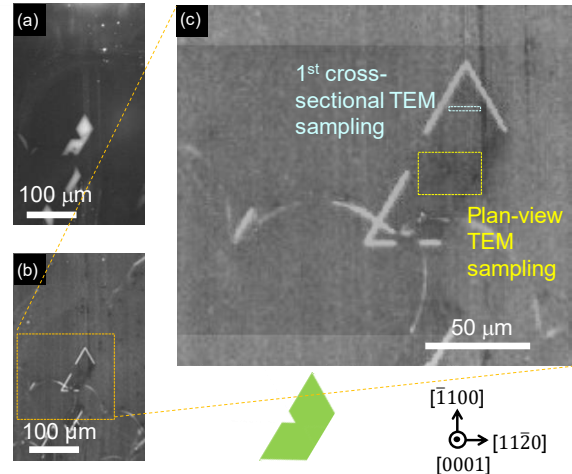
Fig. 3 PL and composite SEM images of 1SSF-B: (a) 420 nm BPF, (b) 750 nm HPF, and (c) composite of (b) and an SEM image.
