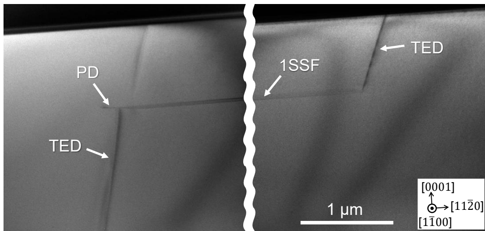
Fig.7 2 nd cross-sectional BF-TEM image of 1SSF-B.
