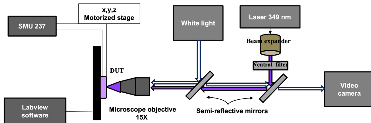
Fig. 1. Schematic representation of the micro-OBIC testbench.
