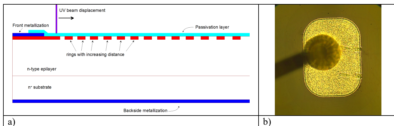
Fig. 2. a) Schematic cross section view of half vertical PiN diodes protected by 22 field rings (principle is sketched here only with 13 rings), b) photograph of the diode with the 50\ \mu\text{m} (diameter) gold ball bonding.
